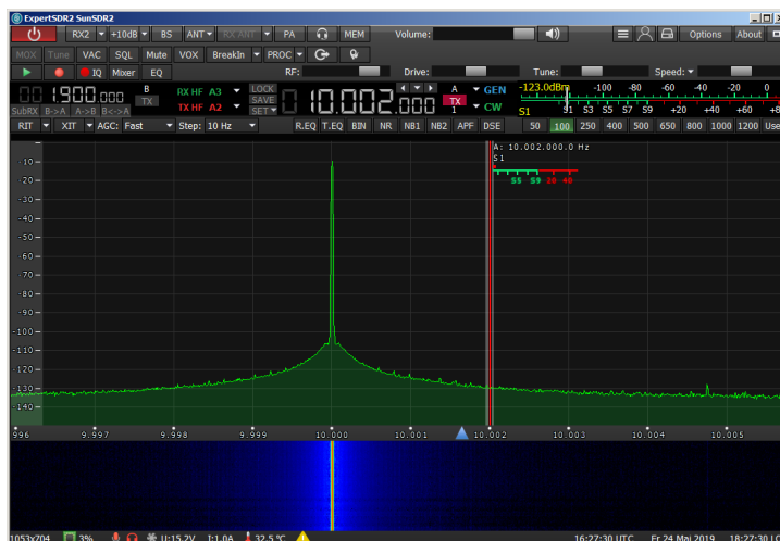
Figure 6: Measurement of sideband noise
