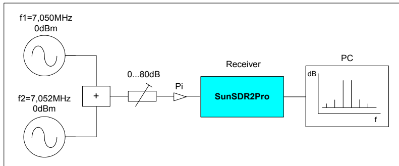
Figure 8: Receiver IMD3 measurement
