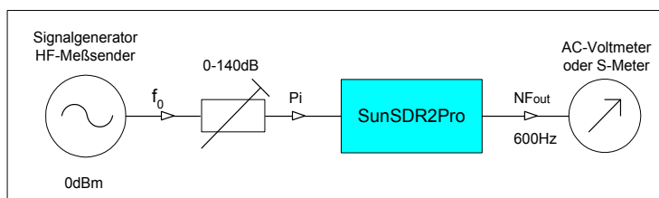
Figure 4: Test setup to determine the sensitivity
