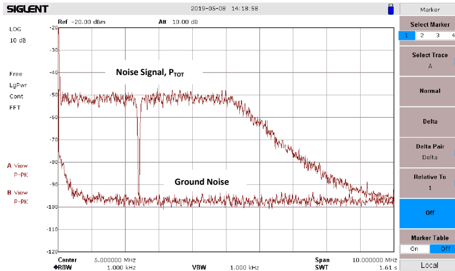
Figure 13: Spectrum at the input of the receiver. Noise signal up to 5MHz, except in the notch filter
