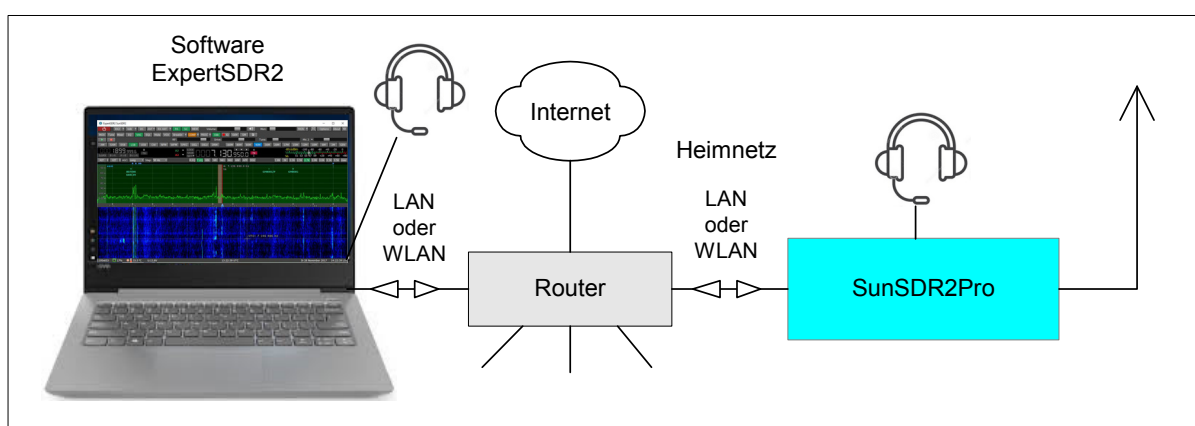
Figure 1: Operation of the SunSDR2Pro in the home network
