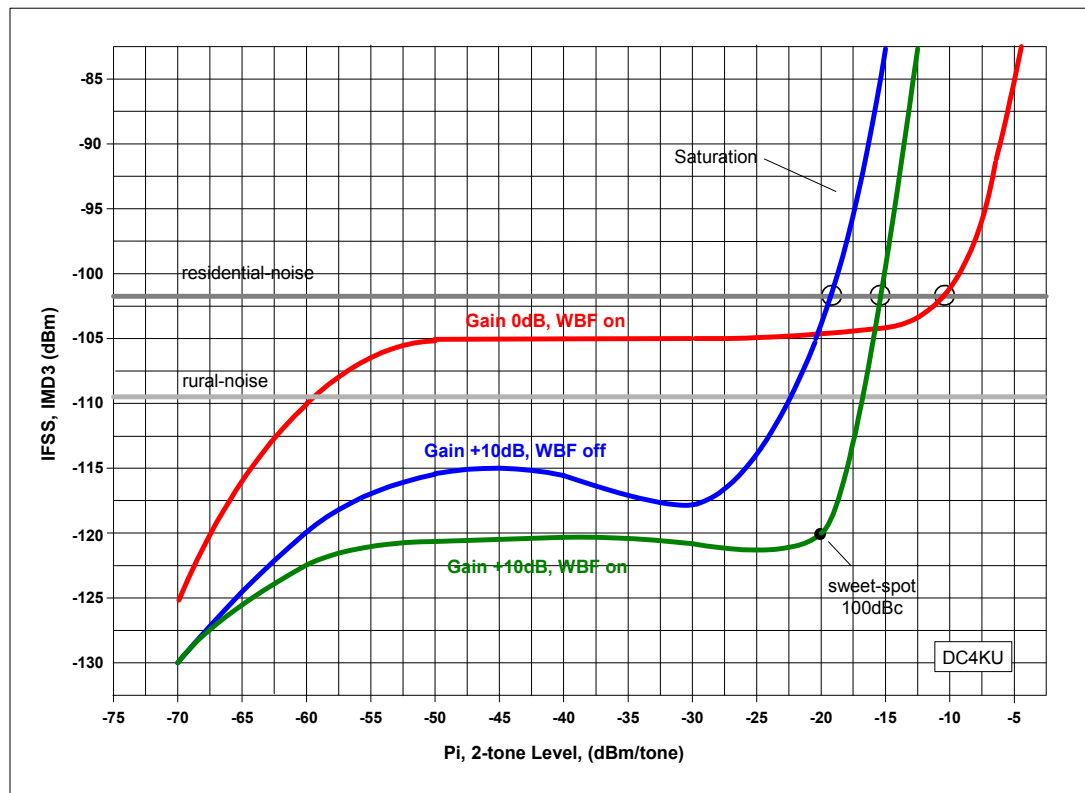
Figure 9: IMD3
