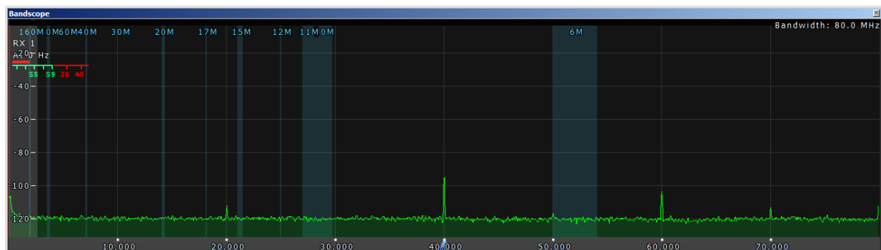
Bild 17: Receiver Spurious Signals from 0-80MHz
