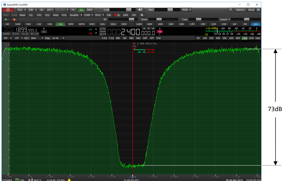
Bild 14: Noise Power Ratio = 73dB
