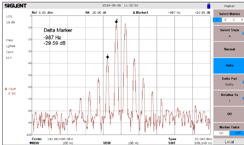
Fig 22: f=145MHz, 7.7Watt PEP, Delta IMD3 = 29,6dB
