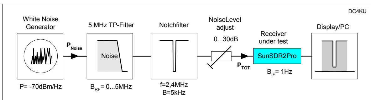
Figure 12: NPR test setup
