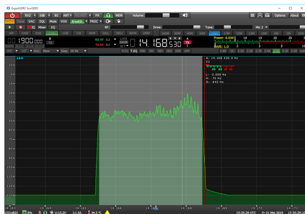
Figure 23: Screen shows the spectrum of the transmission signal
