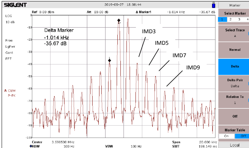
Fig 19: f=3,6\text{MHz} , 20Watt PEP, \text{IMD3}=35,7\text{dBc}
