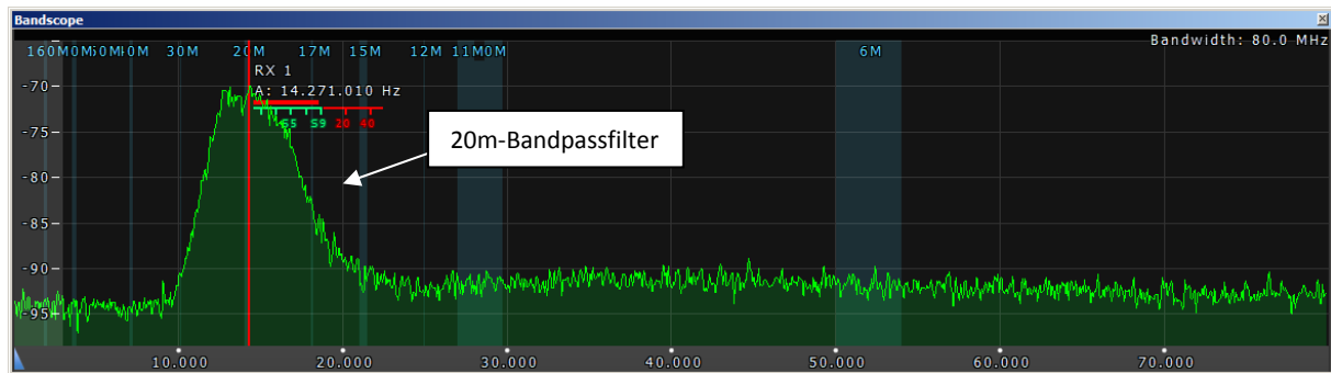
Figure 16: Spectrum with Wide RX filter off. The receiver now automatically selects a suitable, selective BP filter, in the example at 14.2 MHz in the 20 m band.
