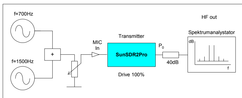
Figure 18: Transmitter IMD3 measurement
