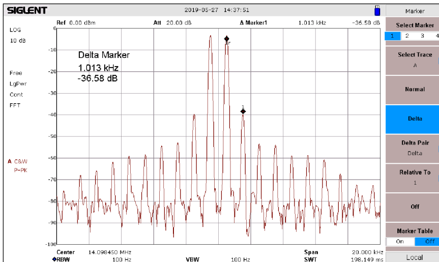
Fig 20: f=14,1\text{MHz} , 18.7Watt PEP, Delta \text{IMD3} = 36,6\text{dBc}
