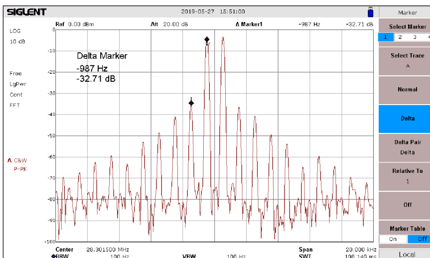
Fig 21: f= 28.3\text{MHz} , 18Watt PEP, Delta \text{IMD3} = 32,7\text{dBc}
