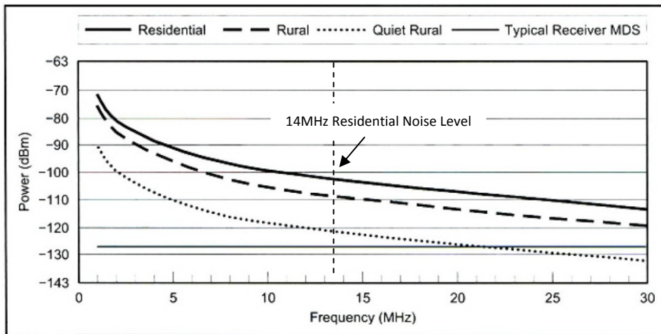
Figure 10: Type. External noise in urban areas (Residential, Urban) and in rural residential areas (Rural), (Man-Made Noise in 500Hz bandwidth, from Rec. ITU-R P.372-7, Radio Noise, ARRL Handbook)
